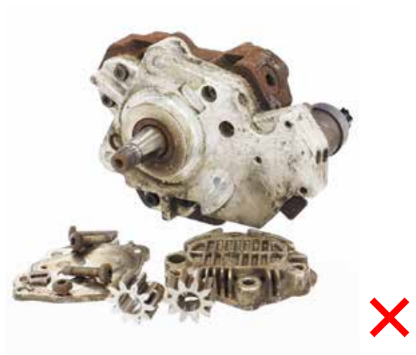
Damaged drive shaft
