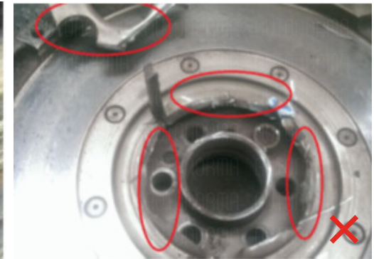
Damaged gearing
