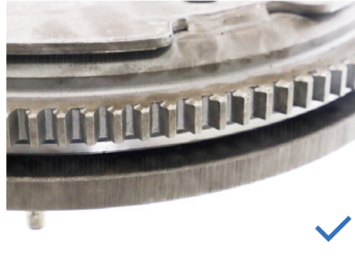
Undamaged gearing
