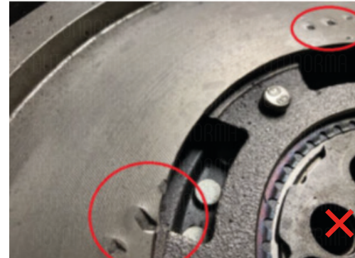
Dent on the friction surface
